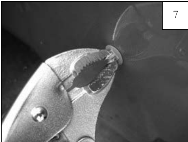
Remove two clips from front using vise grips, pulling with a rocking motion. See step 8.
